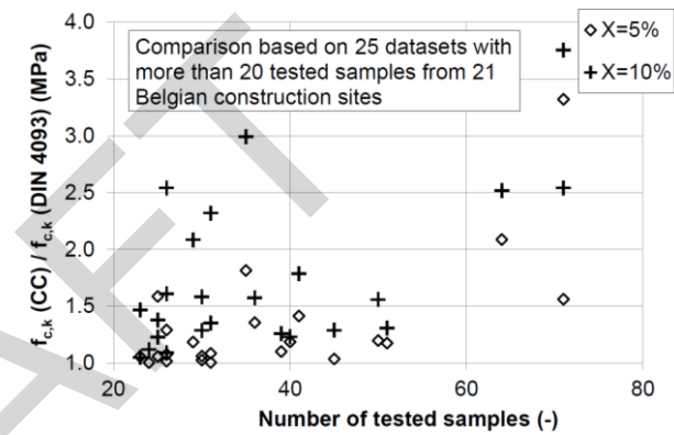
Figure 3. Ratio of the characteristic values ( f_{c,k} (CC) and f_{c,k} (DIN4093)) as a function of the number of tested samples.
